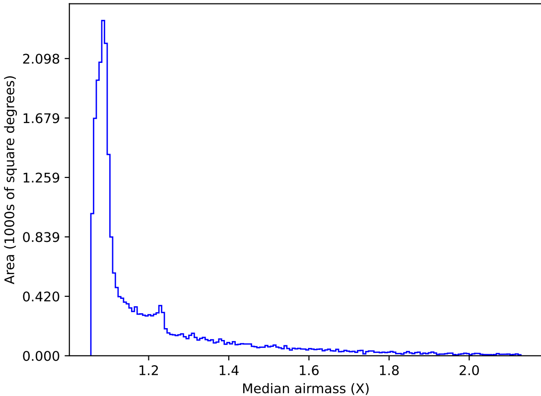
retro_baseline_v2.0_10yrs All sky i band: Median airmass
