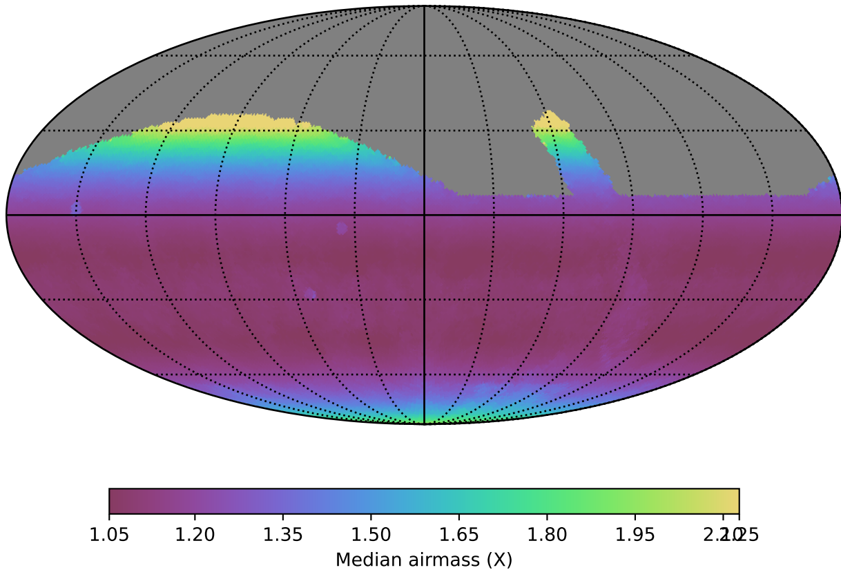
retro_baseline_v2.0_10yrs All sky g band: Median airmass
