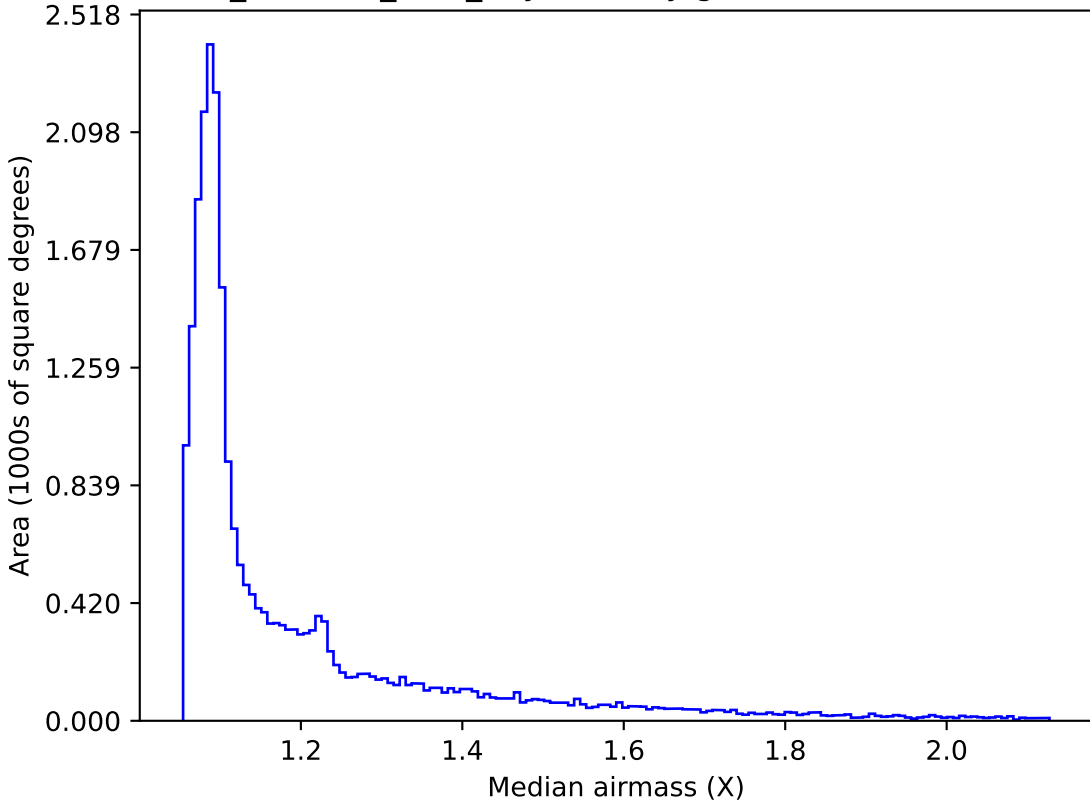
retro_baseline_v2.0_10yrs All sky g band: Median airmass
