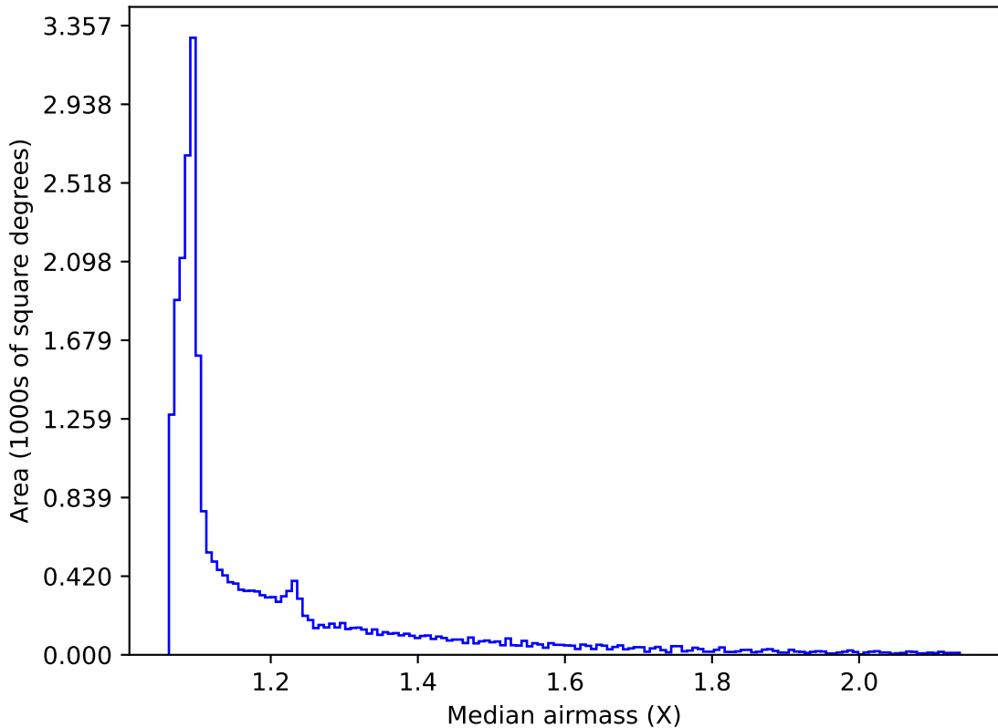
retro_baseline_v2.0_10yrs All sky all bands: Median airmass
