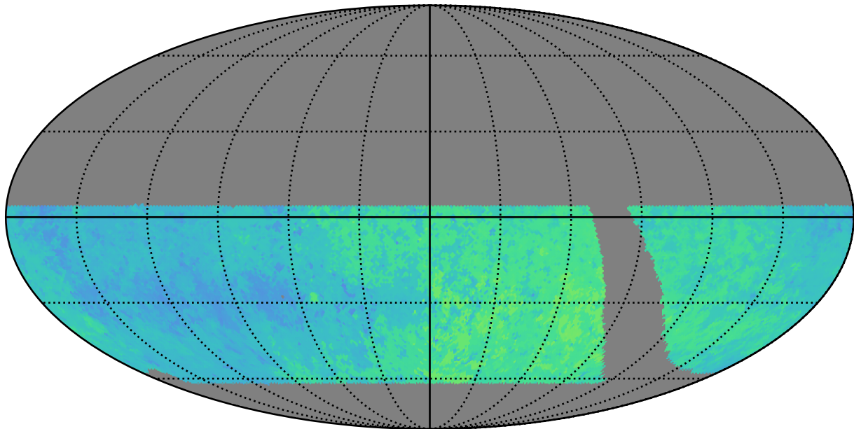
retro_baseline_v2.0_10yrs WFD z band: Median Season Length
