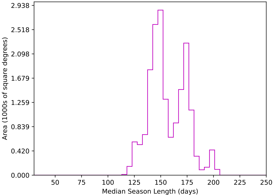
retro_baseline_v2.0_10yrs WFD z band: Median Season Length
