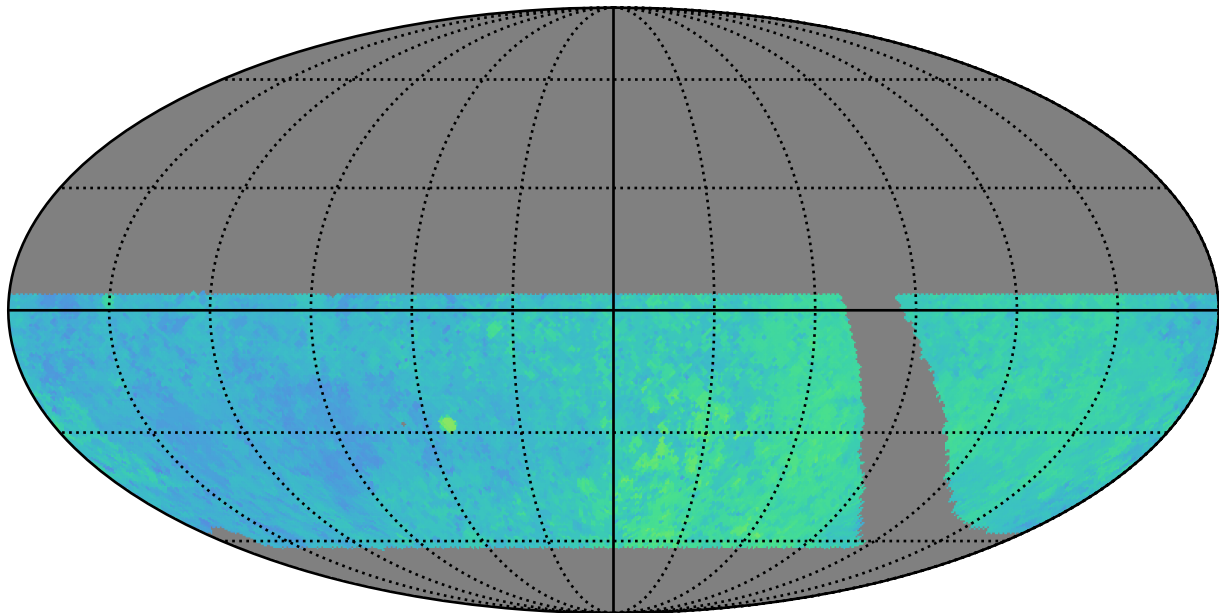
retro_baseline_v2.0_10yrs WFD r band: Median Season Length
