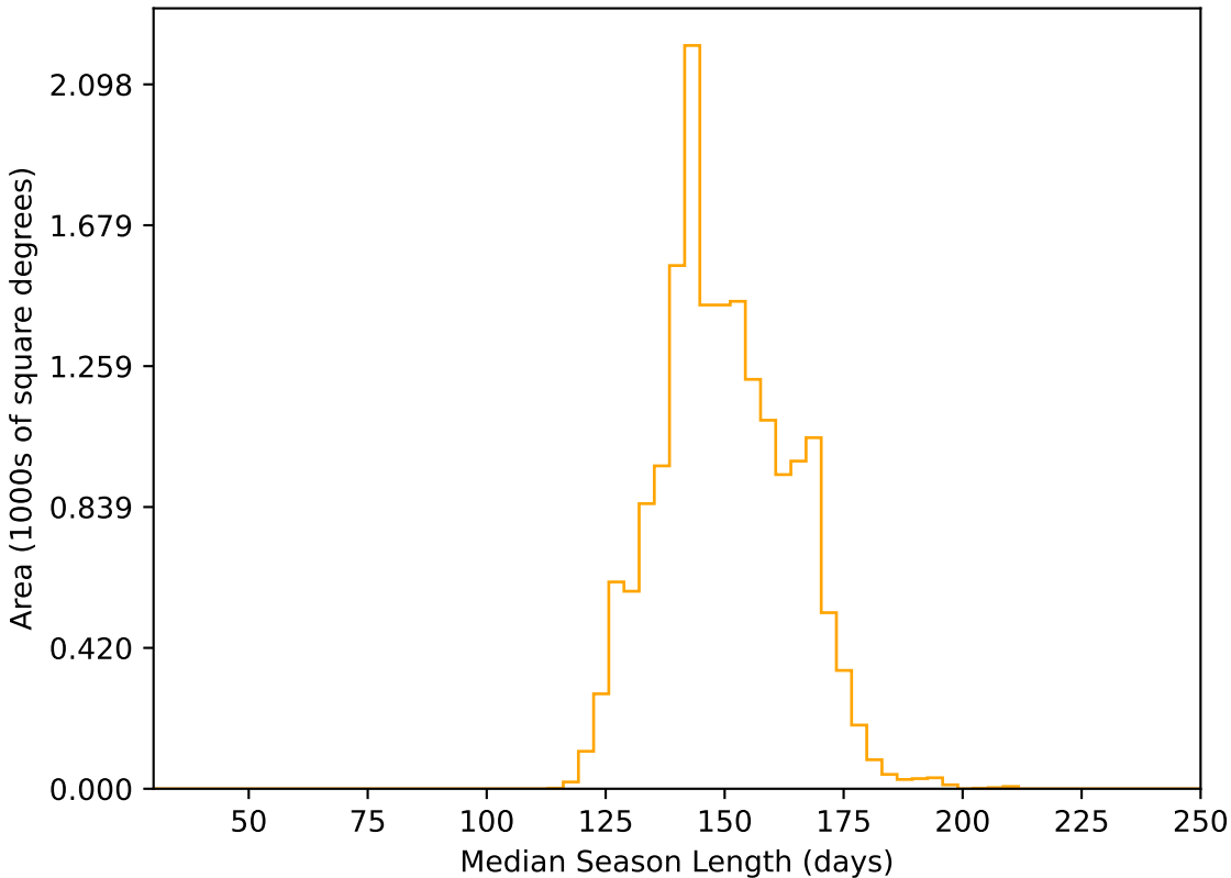
retro_baseline_v2.0_10yrs WFD r band: Median Season Length
