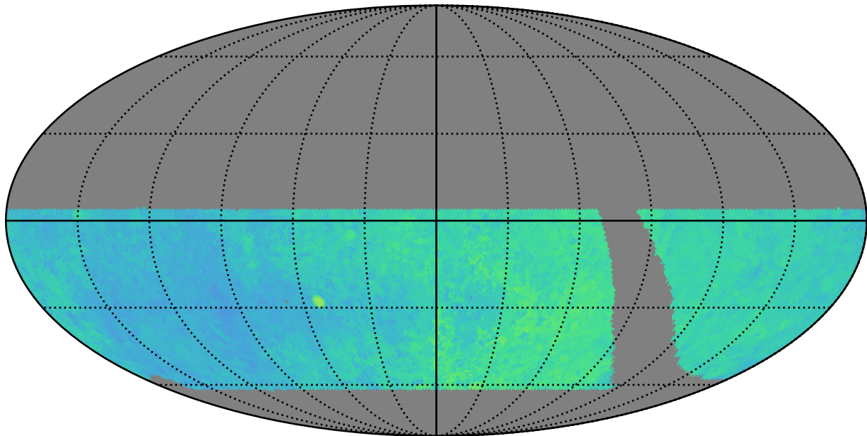
retro_baseline_v2.0_10yrs WFD i band: Median Season Length
