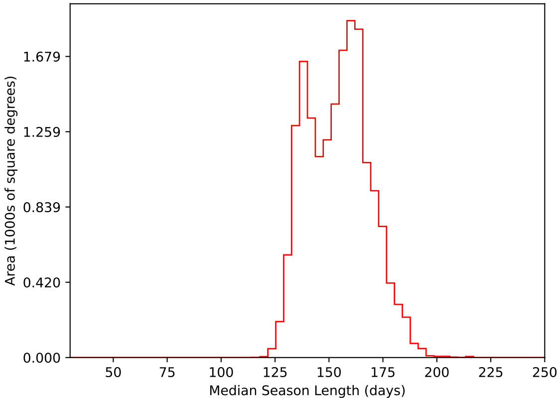
retro_baseline_v2.0_10yrs WFD i band: Median Season Length
