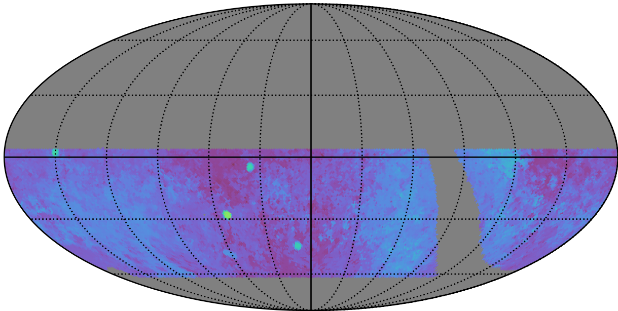
retro_baseline_v2.0_10yrs WFD g band: Median Season Length
