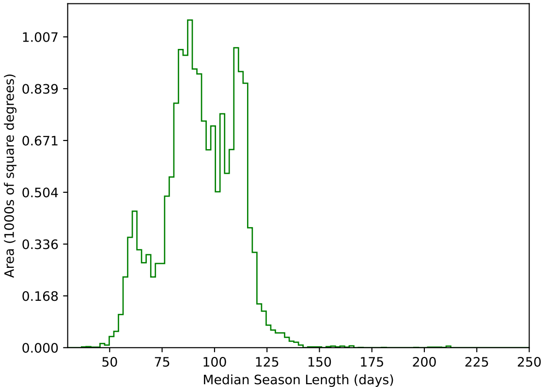
retro_baseline_v2.0_10yrs WFD g band: Median Season Length
