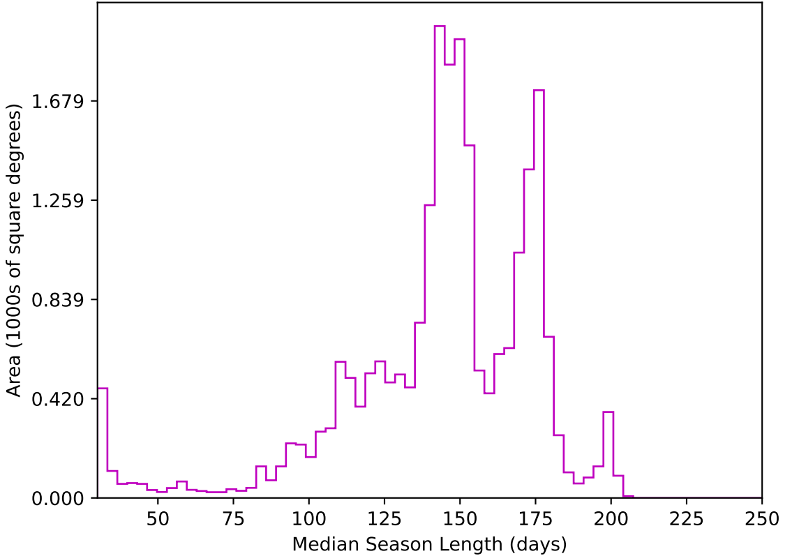
retro_baseline_v2.0_10yrs All sky z band: Median Season Length
