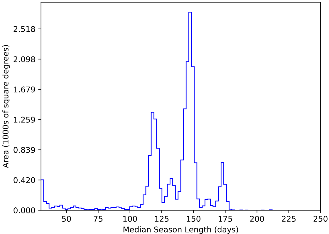
retro_baseline_v2.0_10yrs All sky y band: Median Season Length
