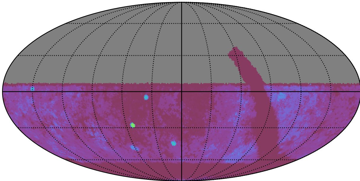
retro_baseline_v2.0_10yrs All sky u band: Median Season Length
