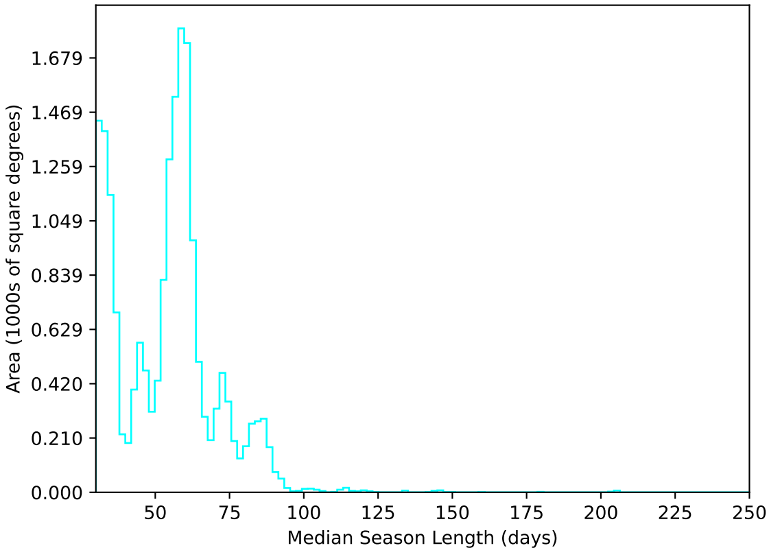
retro_baseline_v2.0_10yrs All sky u band: Median Season Length
