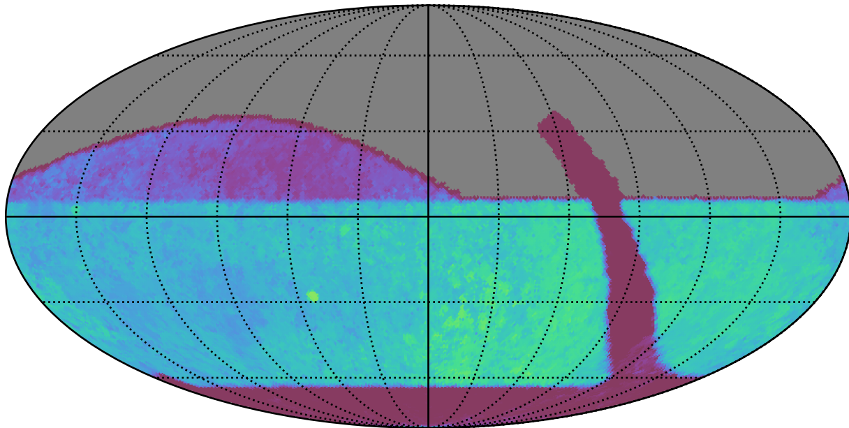
retro_baseline_v2.0_10yrs All sky r band: Median Season Length
