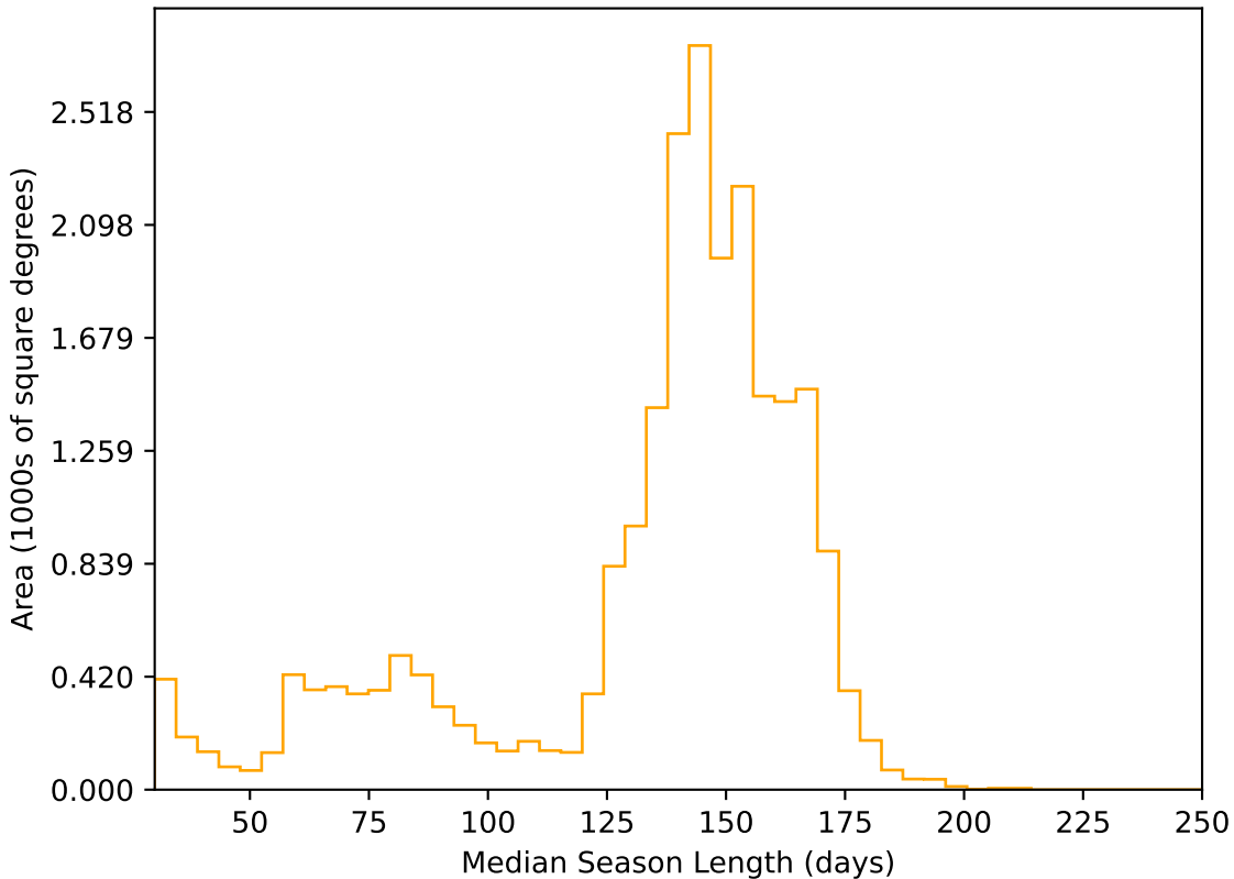
retro_baseline_v2.0_10yrs All sky r band: Median Season Length
