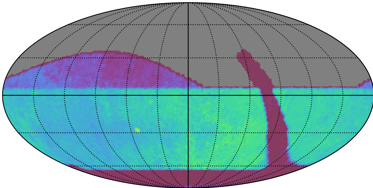
retro_baseline_v2.0_10yrs All sky i band: Median Season Length
