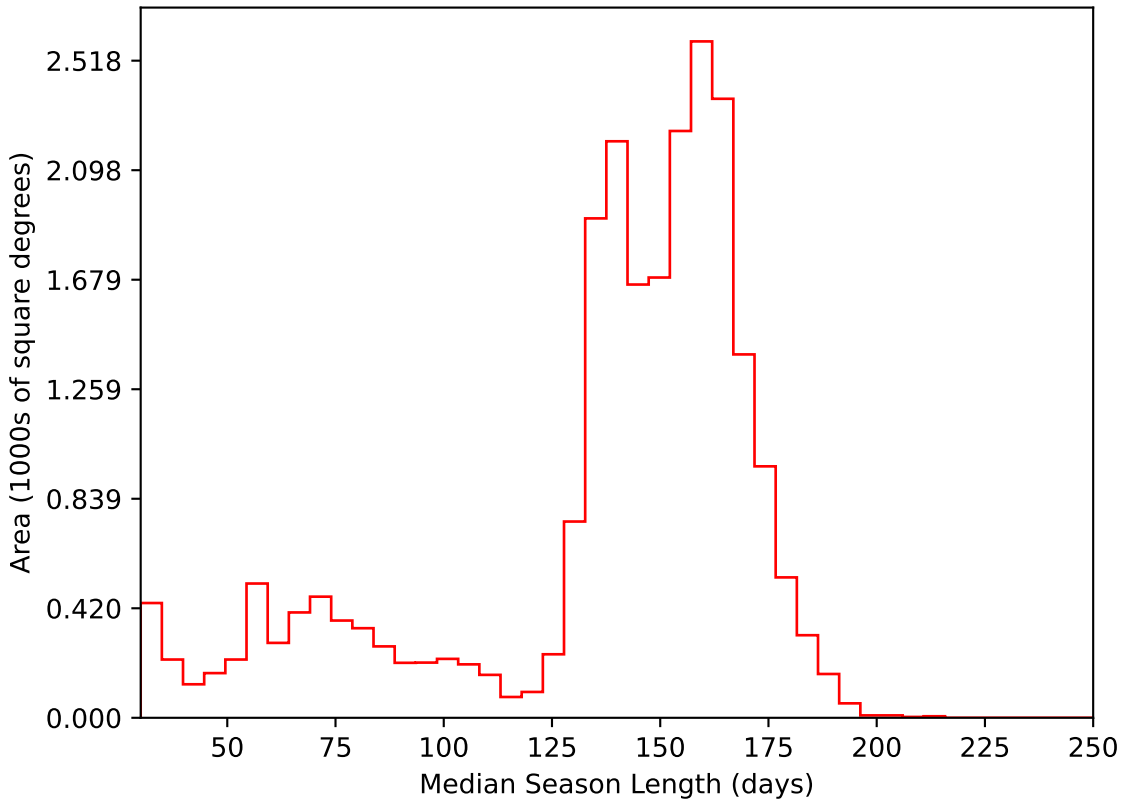
retro_baseline_v2.0_10yrs All sky i band: Median Season Length
