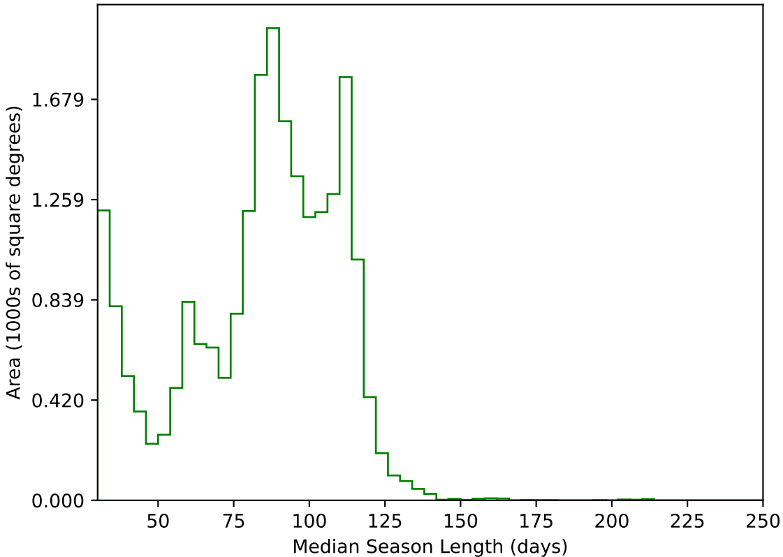
retro_baseline_v2.0_10yrs All sky g band: Median Season Length
