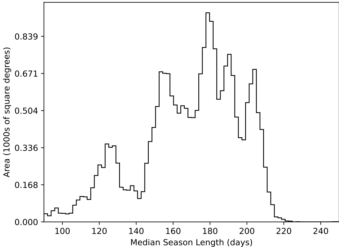
retro_baseline_v2.0_10yrs All sky all bands: Median Season Length
