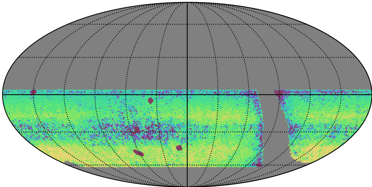
retro_baseline_v2.0_10yrs WFD: Median Intra-Night Gap
