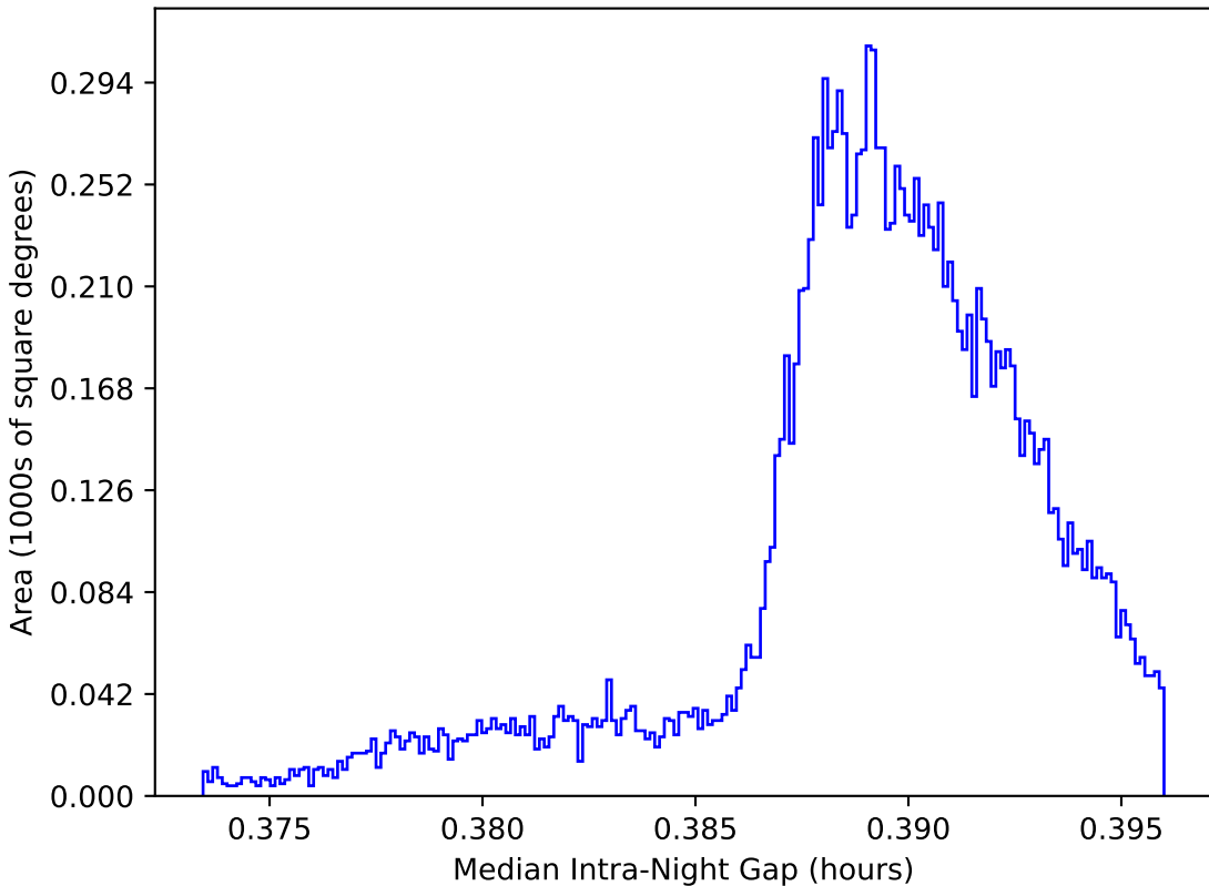
retro_baseline_v2.0_10yrs WFD: Median Intra-Night Gap
