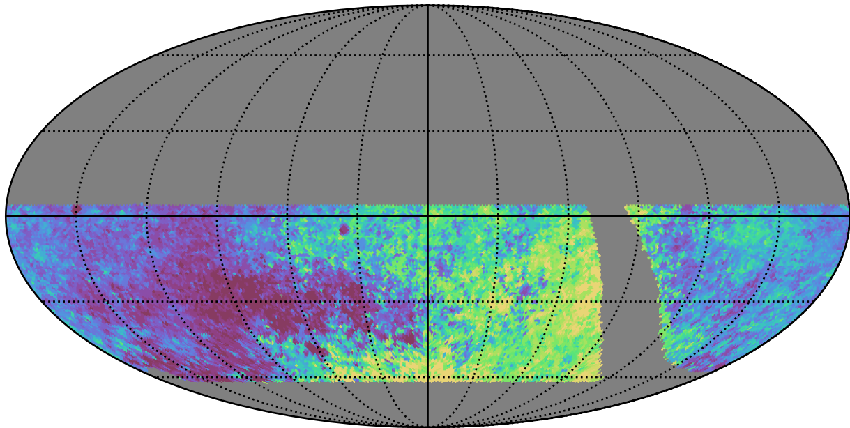
retro_baseline_v2.0_10yrs WFD z band: Median Inter-Night Gap
