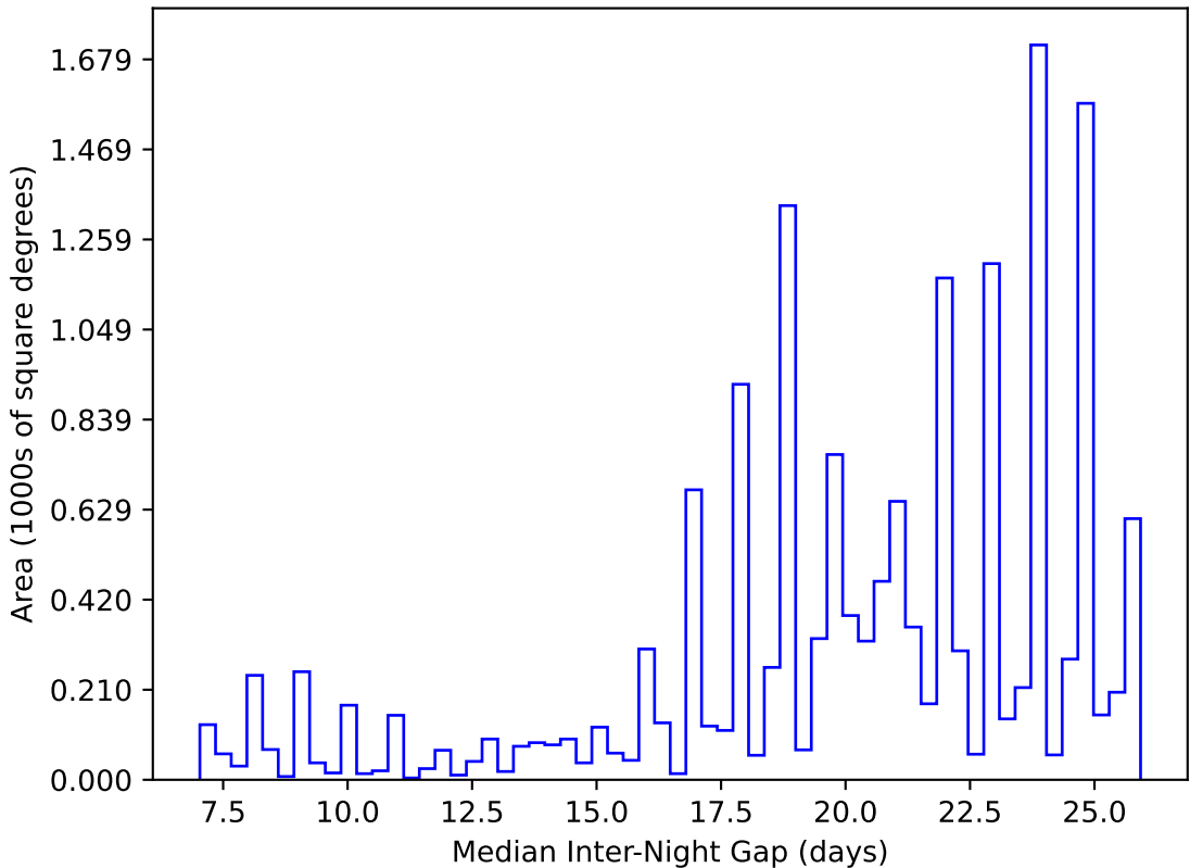
retro_baseline_v2.0_10yrs WFD y band: Median Inter-Night Gap
