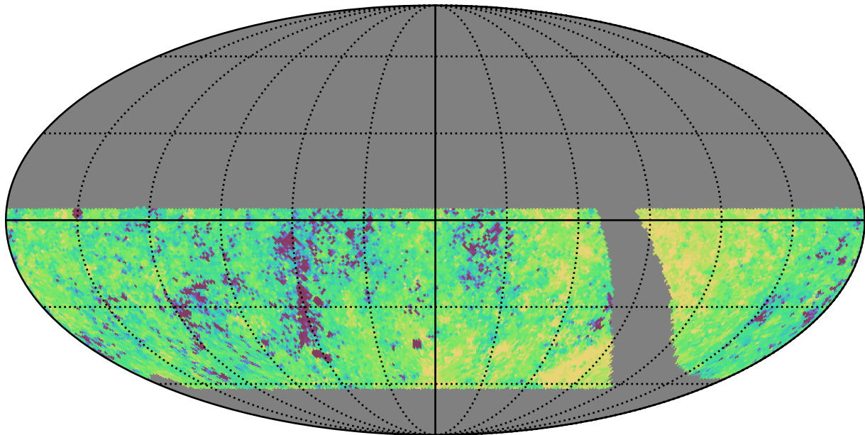
retro_baseline_v2.0_10yrs WFD u band: Median Inter-Night Gap
