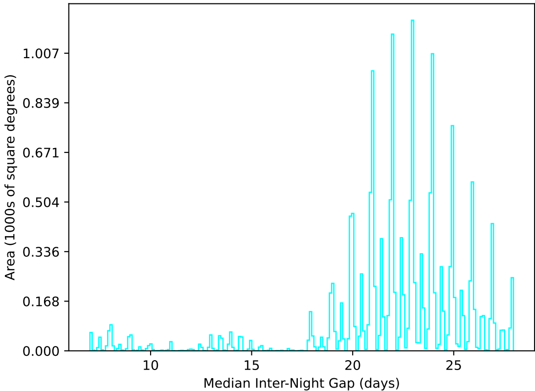
retro_baseline_v2.0_10yrs WFD u band: Median Inter-Night Gap
