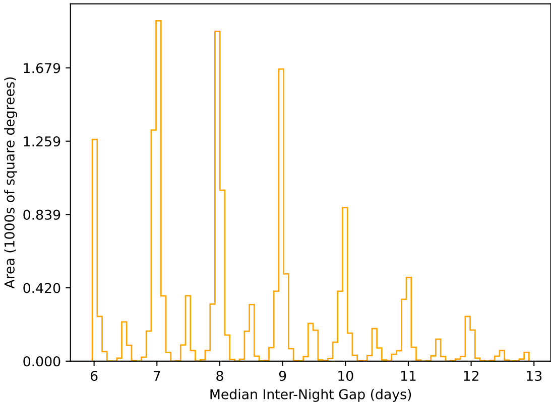
retro_baseline_v2.0_10yrs WFD r band: Median Inter-Night Gap
