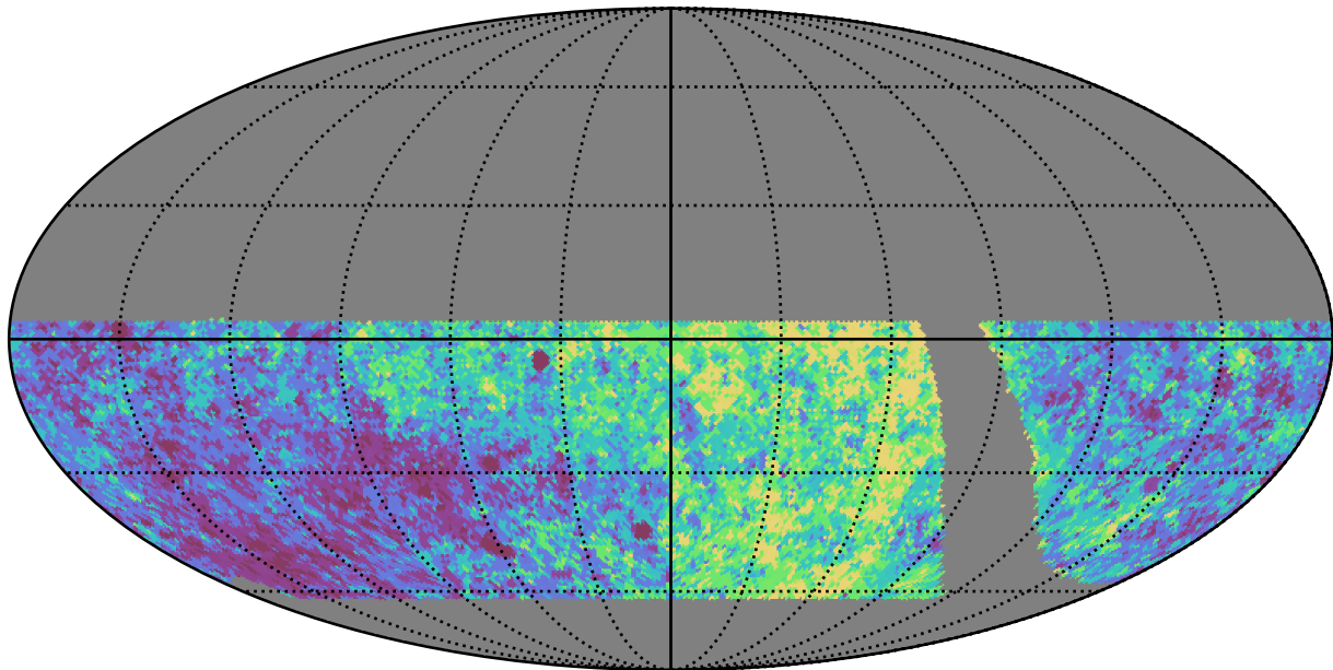
retro_baseline_v2.0_10yrs WFD i band: Median Inter-Night Gap
