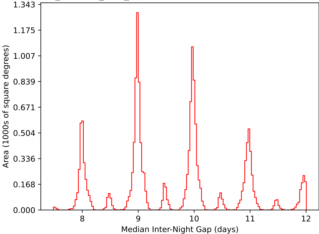
retro_baseline_v2.0_10yrs WFD i band: Median Inter-Night Gap
