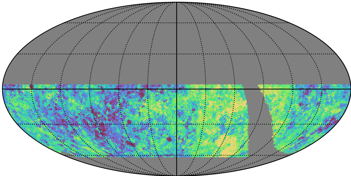
retro_baseline_v2.0_10yrs WFD g band: Median Inter-Night Gap
