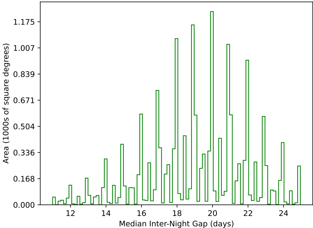
retro_baseline_v2.0_10yrs WFD g band: Median Inter-Night Gap
