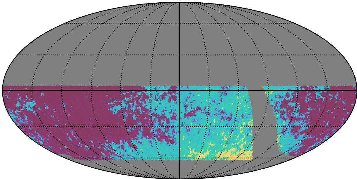
retro_baseline_v2.0_10yrs WFD all bands: Median Inter-Night Gap
