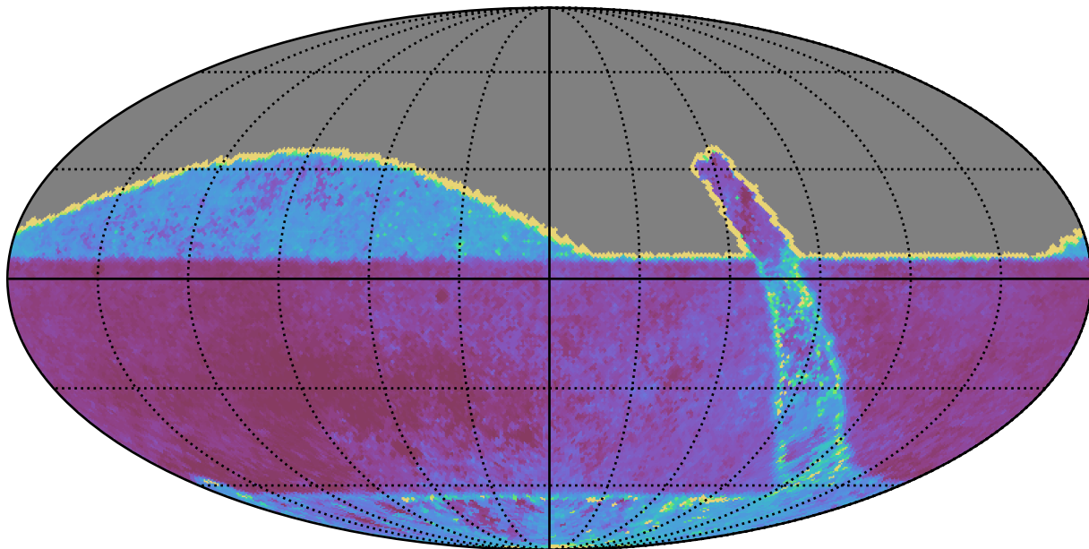
retro_baseline_v2.0_10yrs All sky z band: Median Inter-Night Gap
