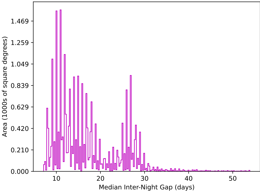
retro_baseline_v2.0_10yrs All sky z band: Median Inter-Night Gap
