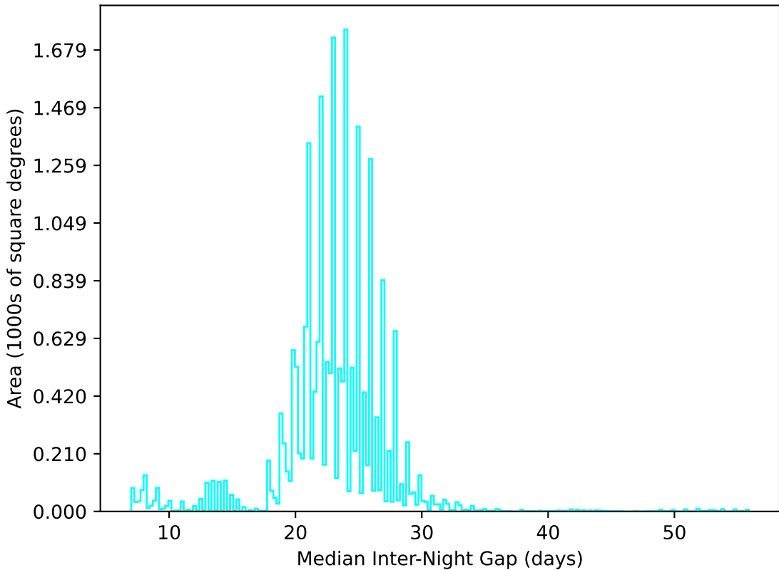
retro_baseline_v2.0_10yrs All sky u band: Median Inter-Night Gap
