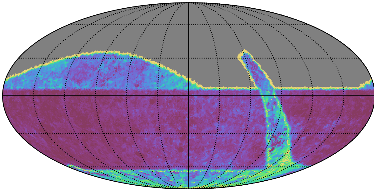
retro_baseline_v2.0_10yrs All sky r band: Median Inter-Night Gap
