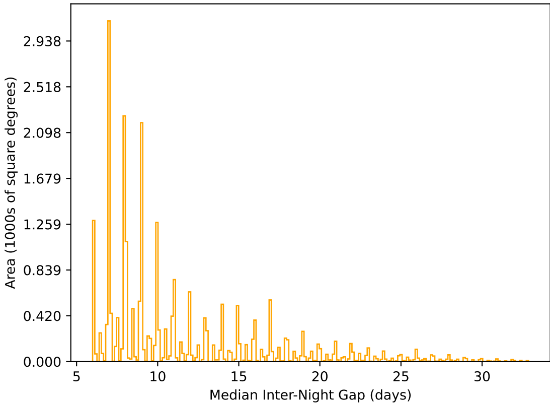
retro_baseline_v2.0_10yrs All sky r band: Median Inter-Night Gap
