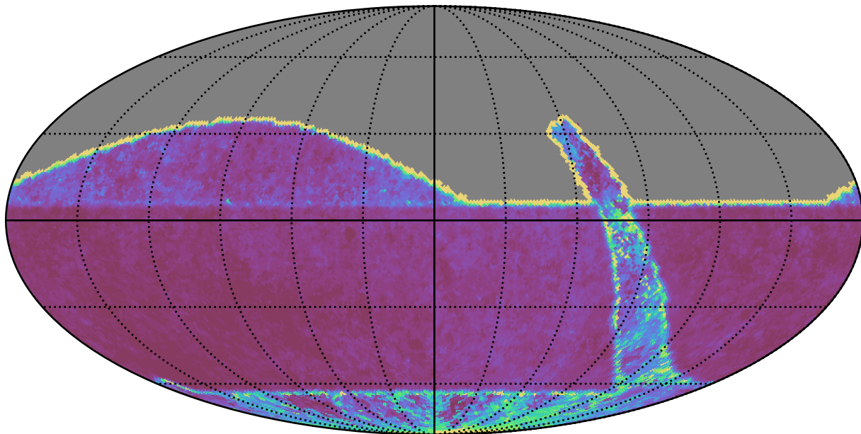
retro_baseline_v2.0_10yrs All sky i band: Median Inter-Night Gap
