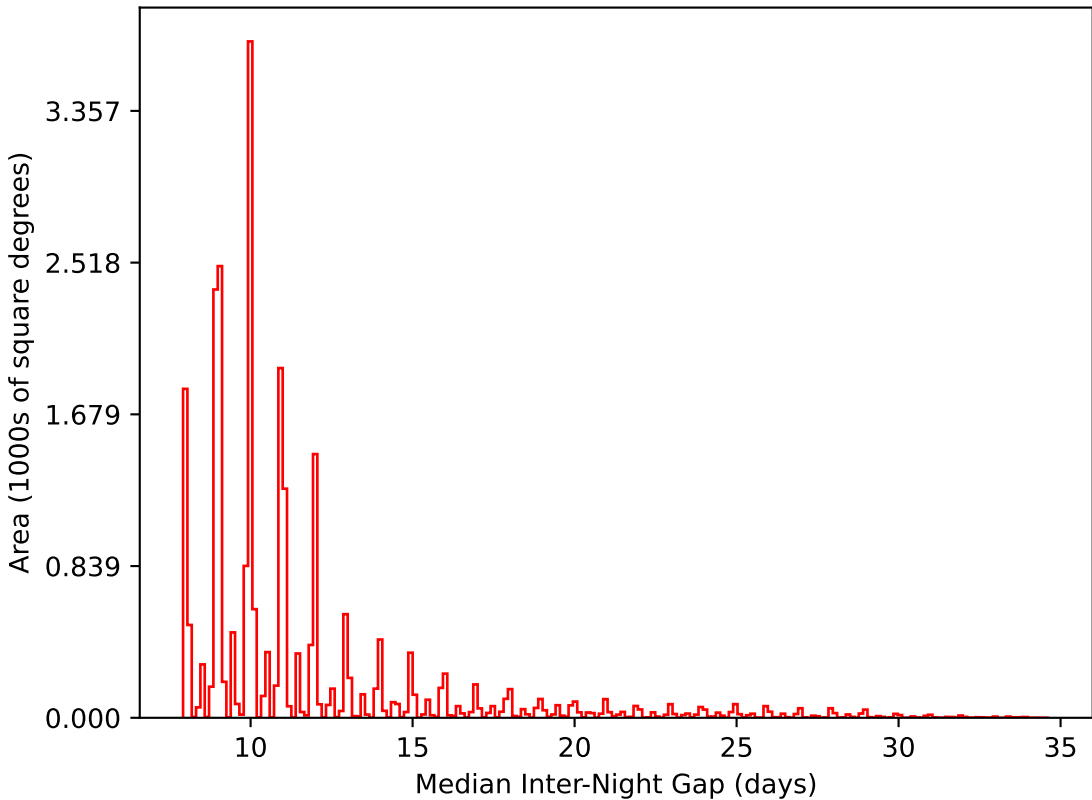
retro_baseline_v2.0_10yrs All sky i band: Median Inter-Night Gap
