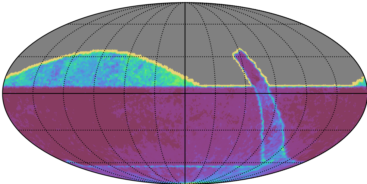
retro_baseline_v2.0_10yrs All sky all bands: Median Inter-Night Gap
