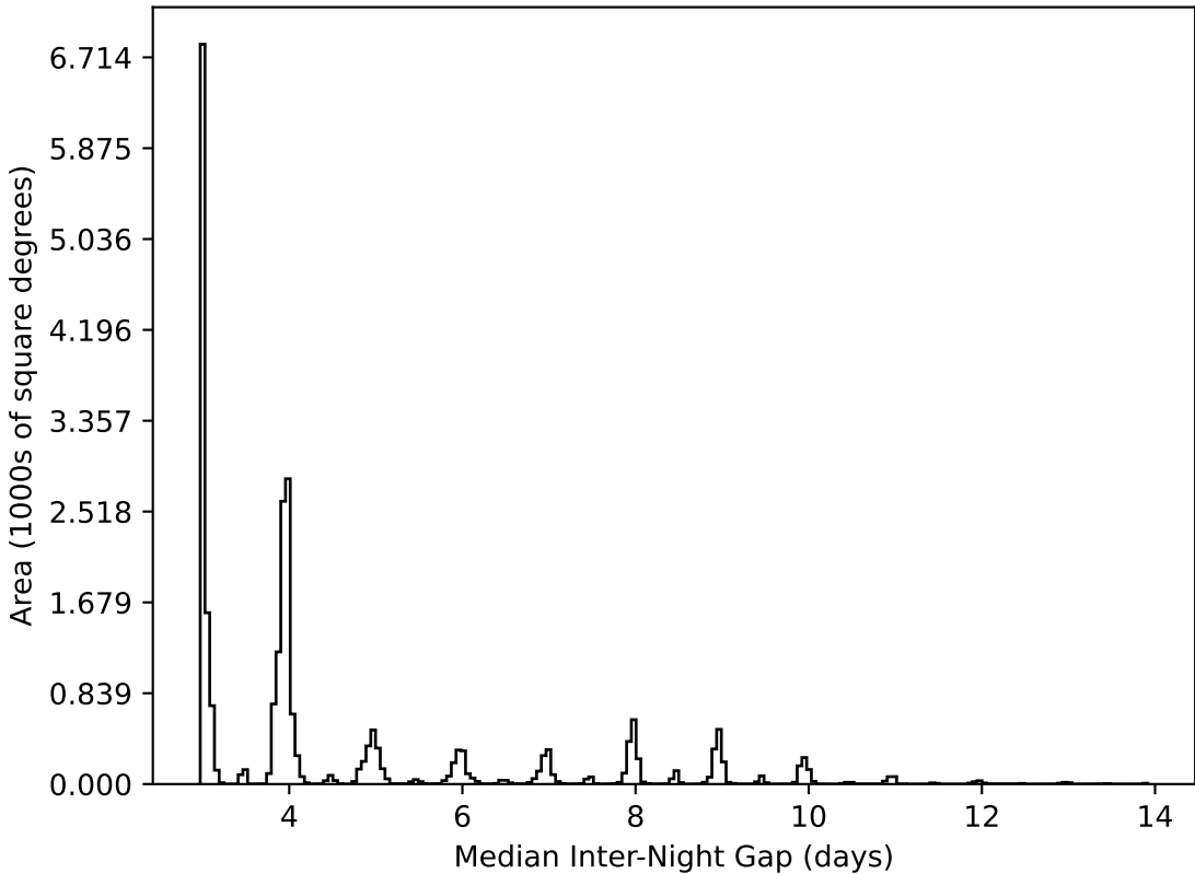
retro_baseline_v2.0_10yrs All sky all bands: Median Inter-Night Gap
