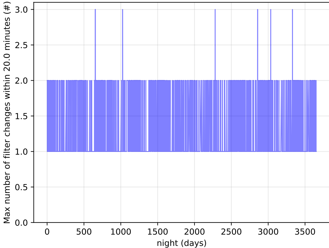
retro_baseline_v2.0_10yrs Per Night: Max number of filter changes within 20.0 minutes
