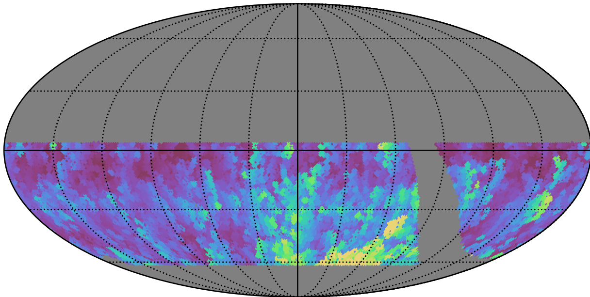
retro_baseline_v2.0_10yrs WFD u band: Max normairmass
