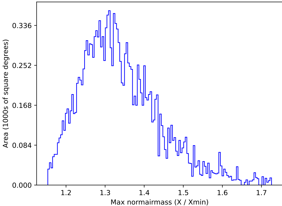
retro_baseline_v2.0_10yrs WFD r band: Max normairmass
