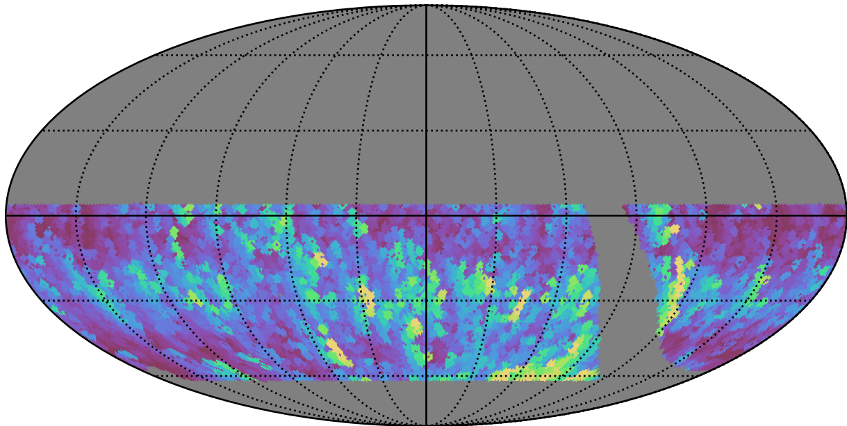
retro_baseline_v2.0_10yrs WFD i band: Max normairmass
