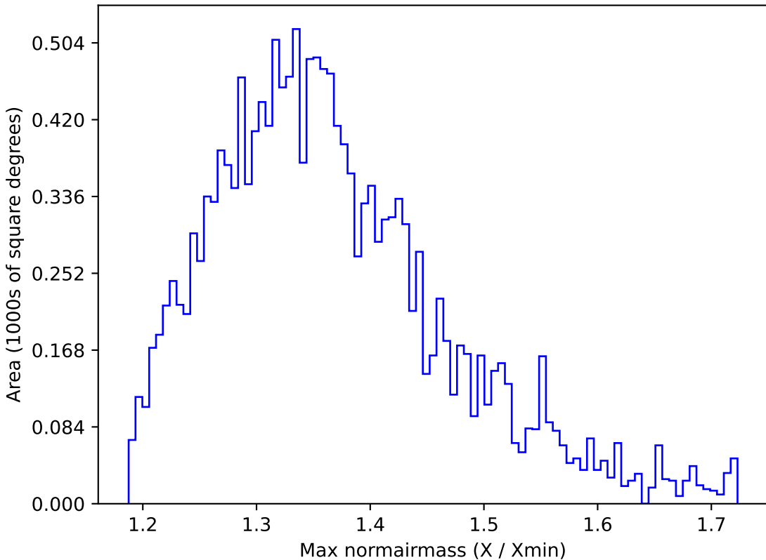
retro_baseline_v2.0_10yrs WFD i band: Max normairmass
