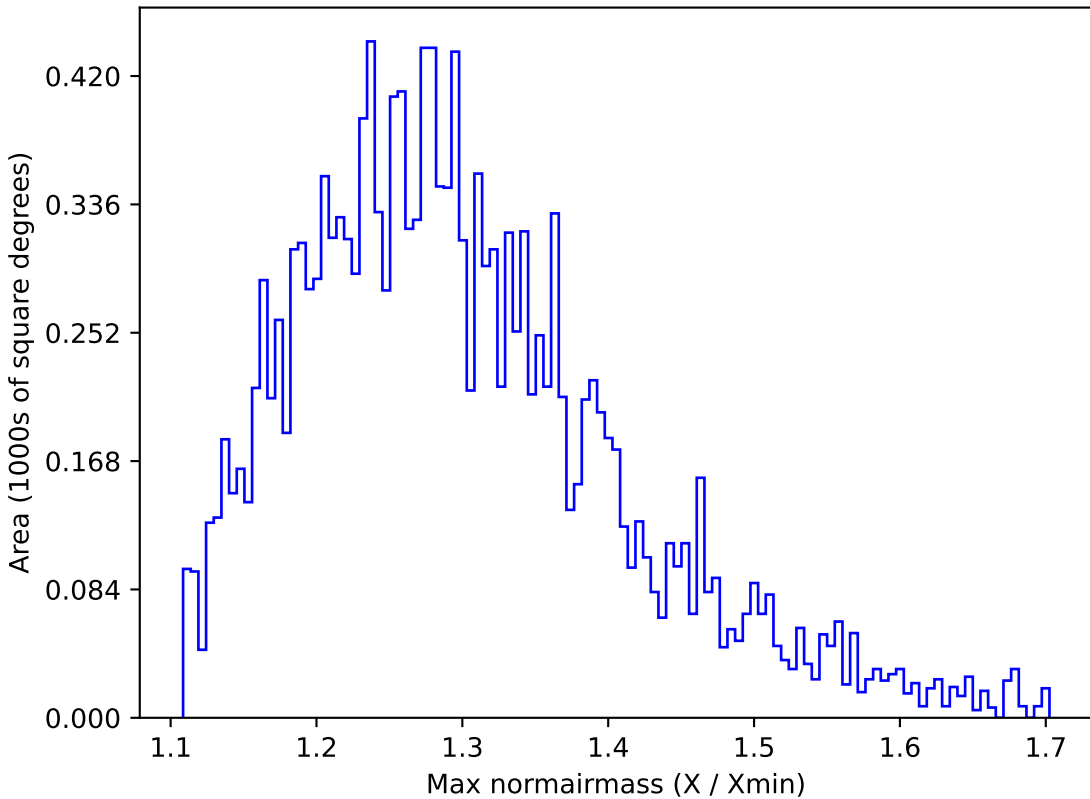
retro_baseline_v2.0_10yrs WFD g band: Max normairmass
