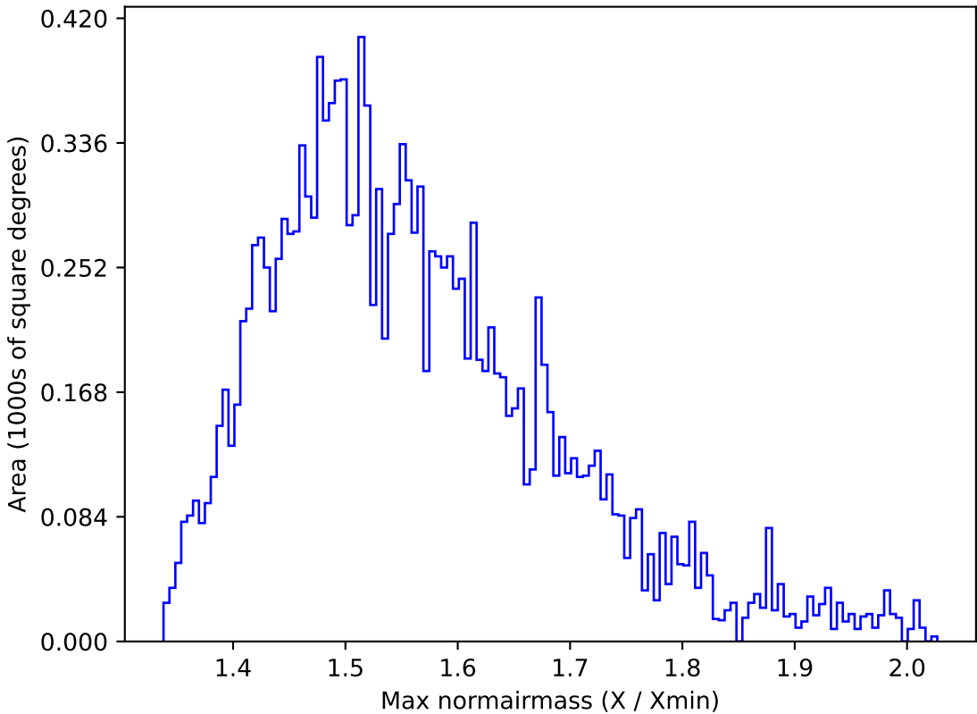
retro_baseline_v2.0_10yrs WFD all bands: Max normairmass
